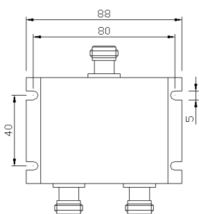
2-way Splitter
