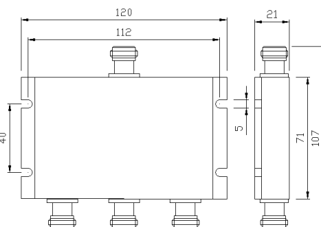
3-way Splitter
