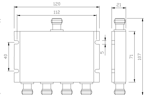
4-way Splitter
